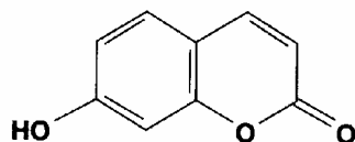
Fig. 6 – Umbelliferone
